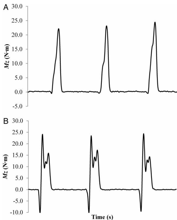
Figure 4 A typical M_z trace from one participant during the 8 km/hour trial during (A) FOR; (B) REV wheelchair propulsion.
