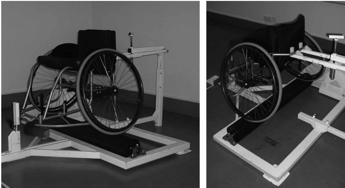
Figure 1 The experimental setup illustrating the single-roller WERG and its interaction with the wheelchair.
