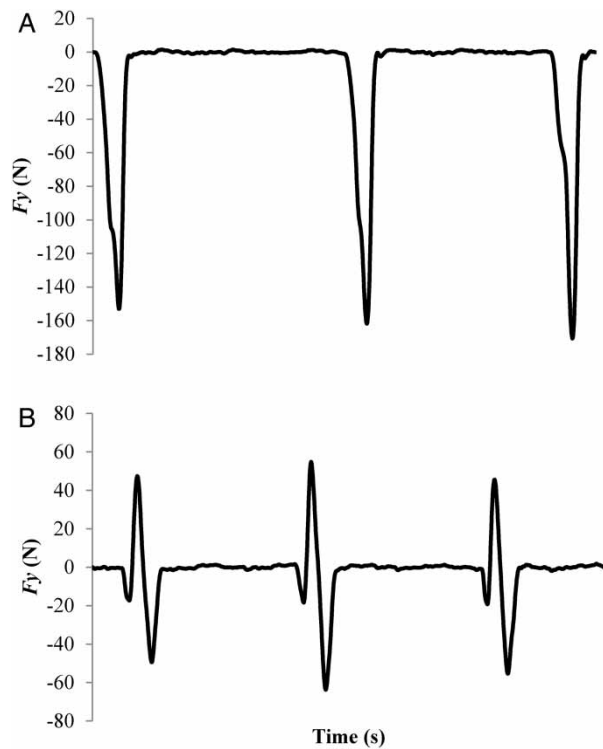
Figure 3 A typical F_y trace from one participant during the 8 km/hour trial during (A) FOR; (B) REV wheelchair propulsion.
